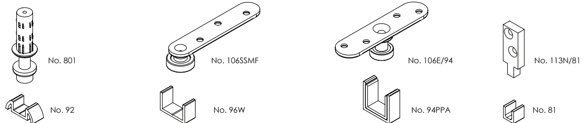
Alternative spring loaded guide & channel
