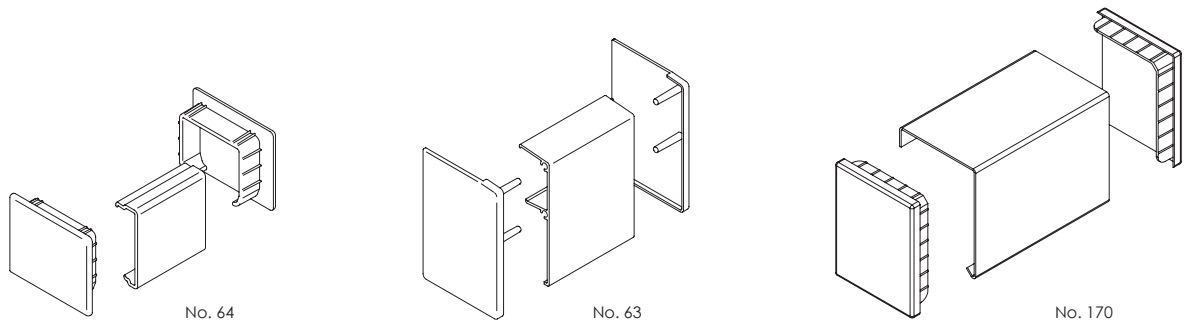
Pelmet and End Caps Zero Clearance 60 Length: 2m or 3m
